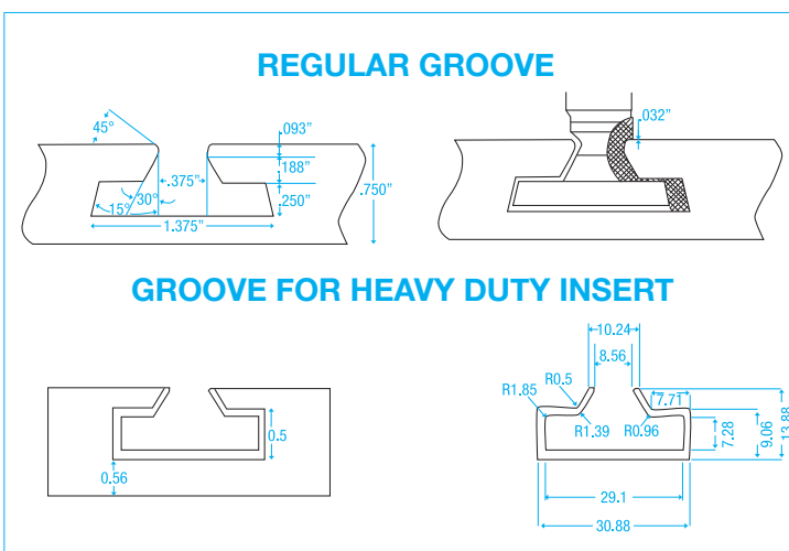
PVC STRIP (Regular Grooves) White • Black • Grey • #U961 • Maple M101 • Others on request
